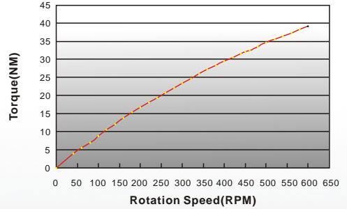
GL-PMG-1000 PMG Input Torque Curve
