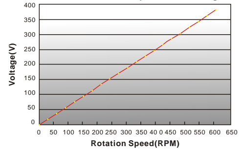
GL-PMG-1000 PMG Open Circuit Voltage
